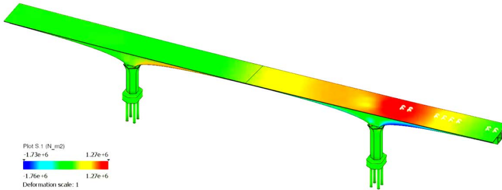
Figure 2. Bridge showing contours of tensile stress along the axis. The tensile stress gets generated due to live load from the train.
